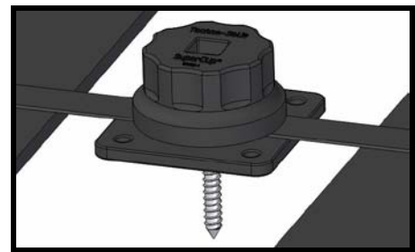
13. SuperClip Installed
